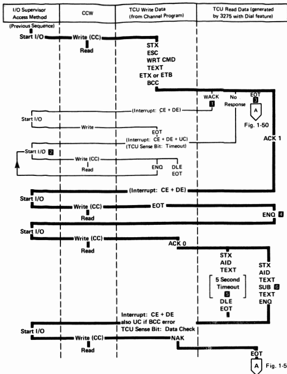
Figure 1-49 (Part 1 of 2). Example of Maintained Connection, Sequence/Response Diagram – Dial Feature
