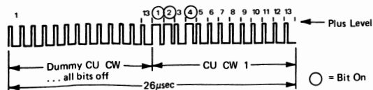
Figure 1-14. CU CW 1 Detected on 3277
