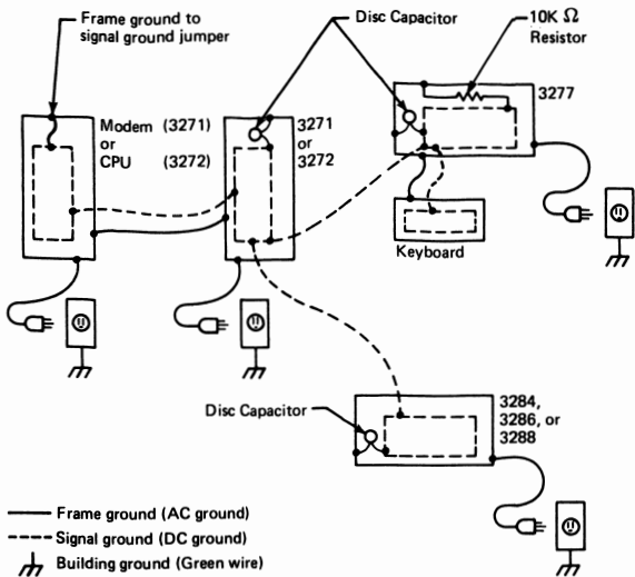
Figure 1-2. 3270 System Grounding
