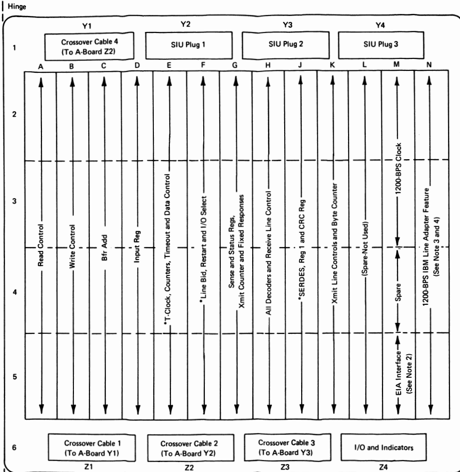
Figure 4-10. 3275 B-Gate Card Layout by Function (Dial)
