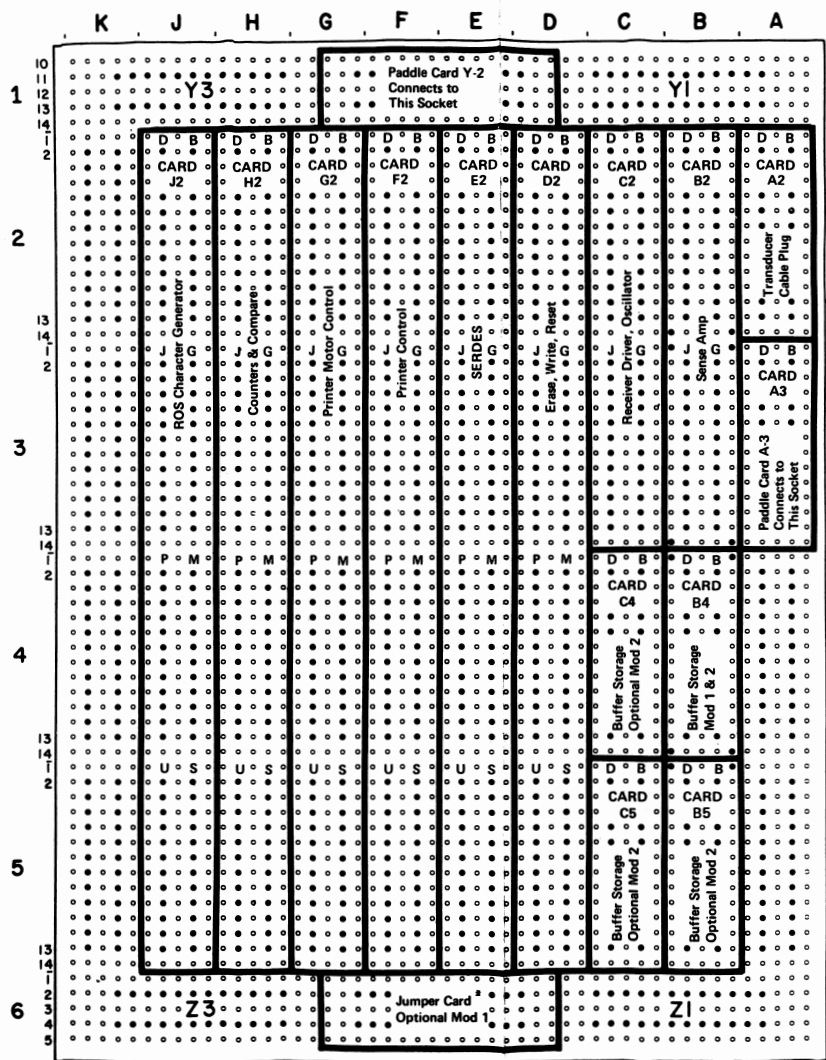
Figure 6-2. 3284/3286 Model 1 and 2 A-Gate Card Layout by Function
