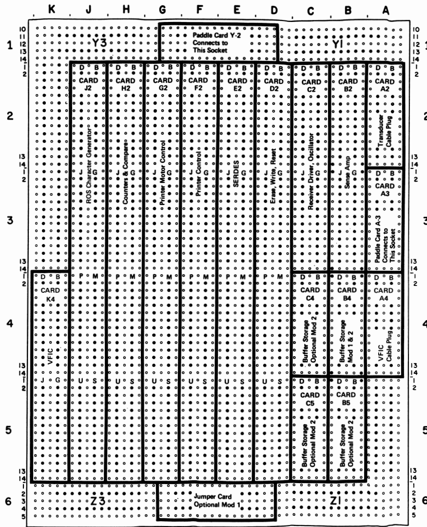
Figure 6-4. 3284/3286 Model 1 and 2 A-Gate Card Layout by Function – VFIC
