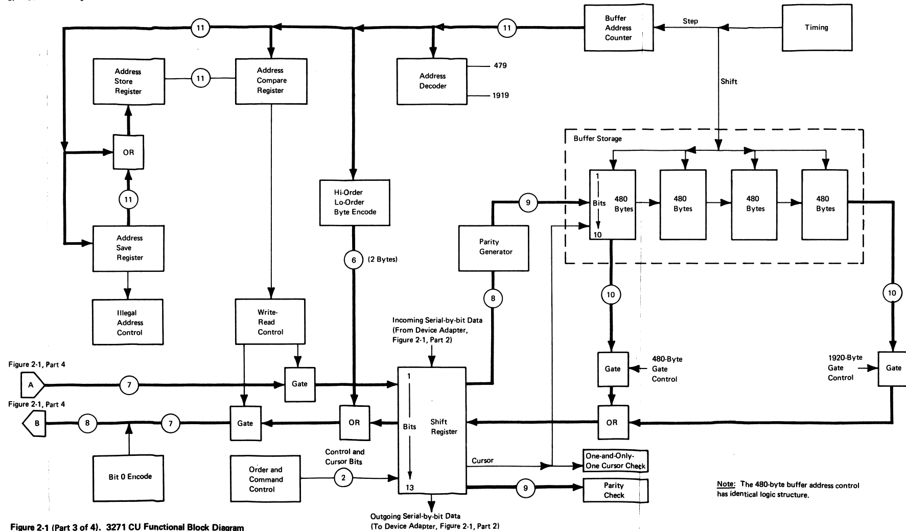
Figure 2-1 (Part 3 of 4). 3271 CU Functional Block Diagram
