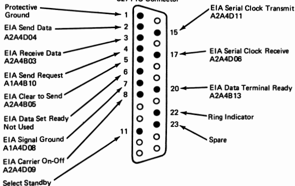
25-Pin Connector Mounted on 3271
