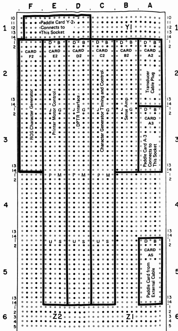
Figure 6-6. 3284/3286 Model 3 A-Gate Card Layout by Function - Dual Case
