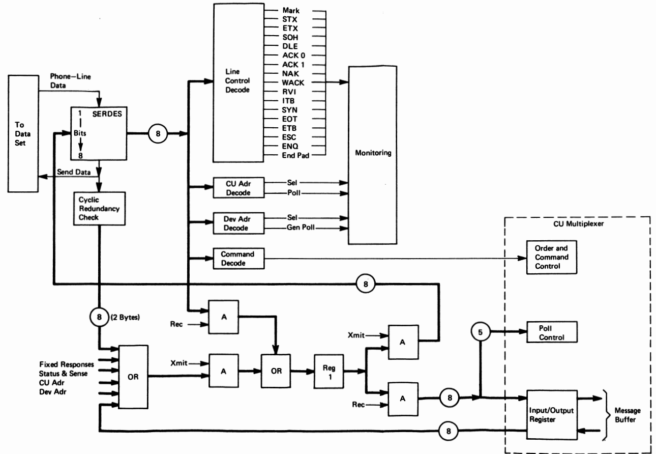
Figure 2-1 (Part 1 of 4). 3271 CU Functional Block Diagram
