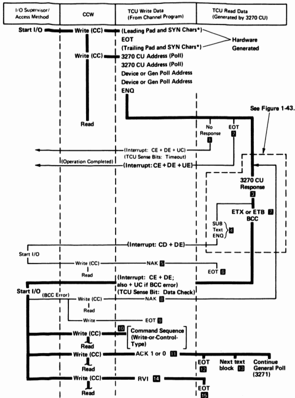
Figure 1-42 (Part 1 of 2). General Poll and Specific Poll, Sequence/Response Diagram
