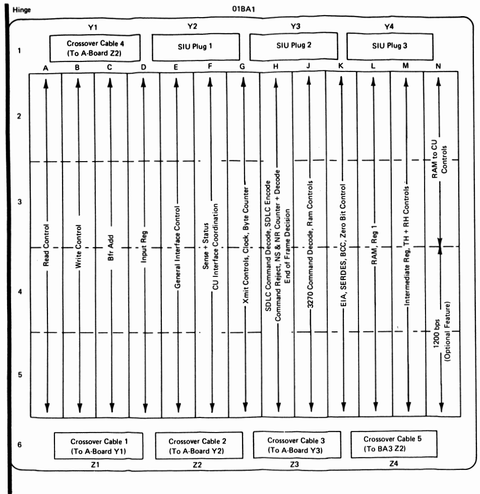
Figure 8-5. 3275 Model 11 and 12 Card Layout by Function – B-Gate
