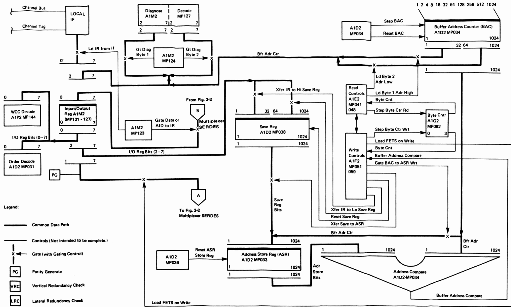
Figure 3-1. 3272 Control Unit Data Flow
