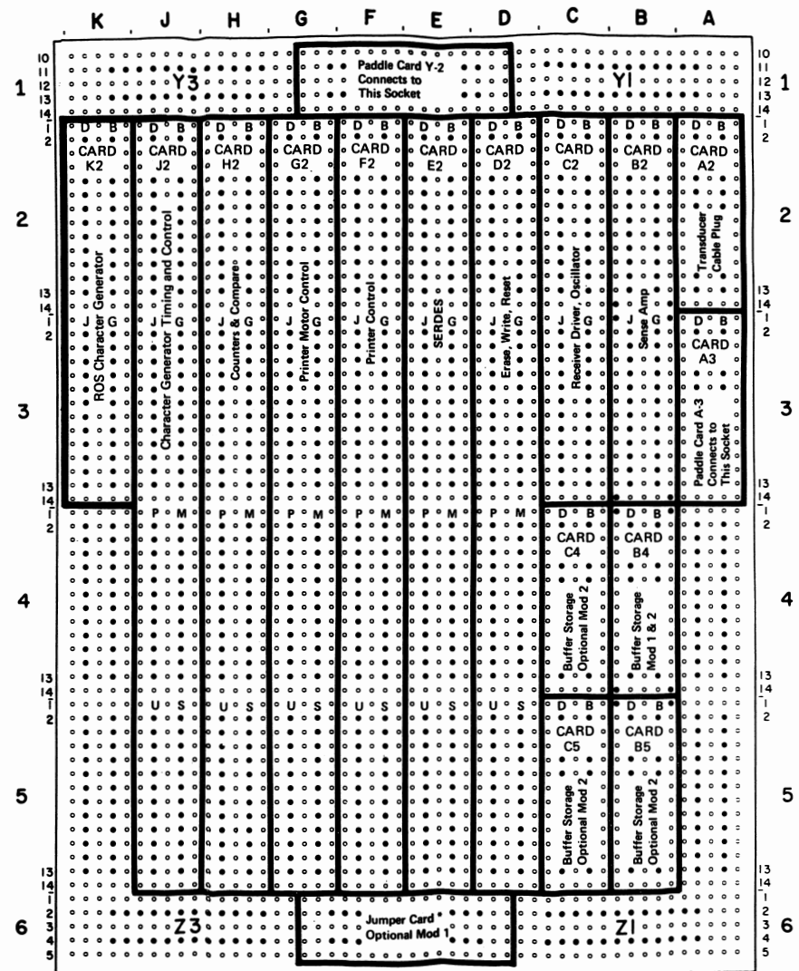
Figure 6-3. 3284/3286 Model 1 and 2 A-Gate Card Layout by Function - Dual Case
