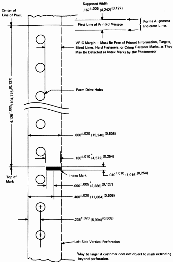
Figure 6-14. VFIC Form, Locations and Dimensions
