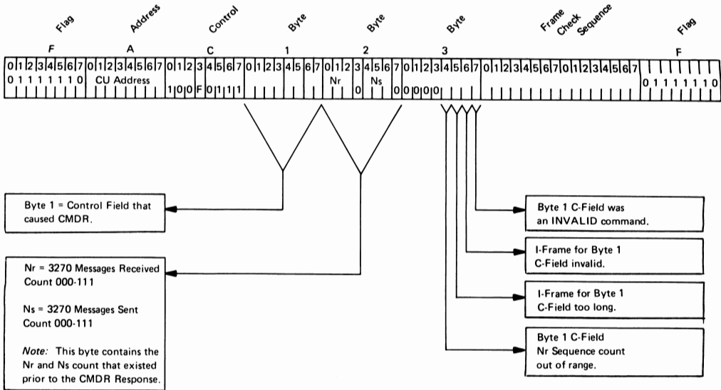
Figure 8-8. Command Reject (CMDR) Message Format
