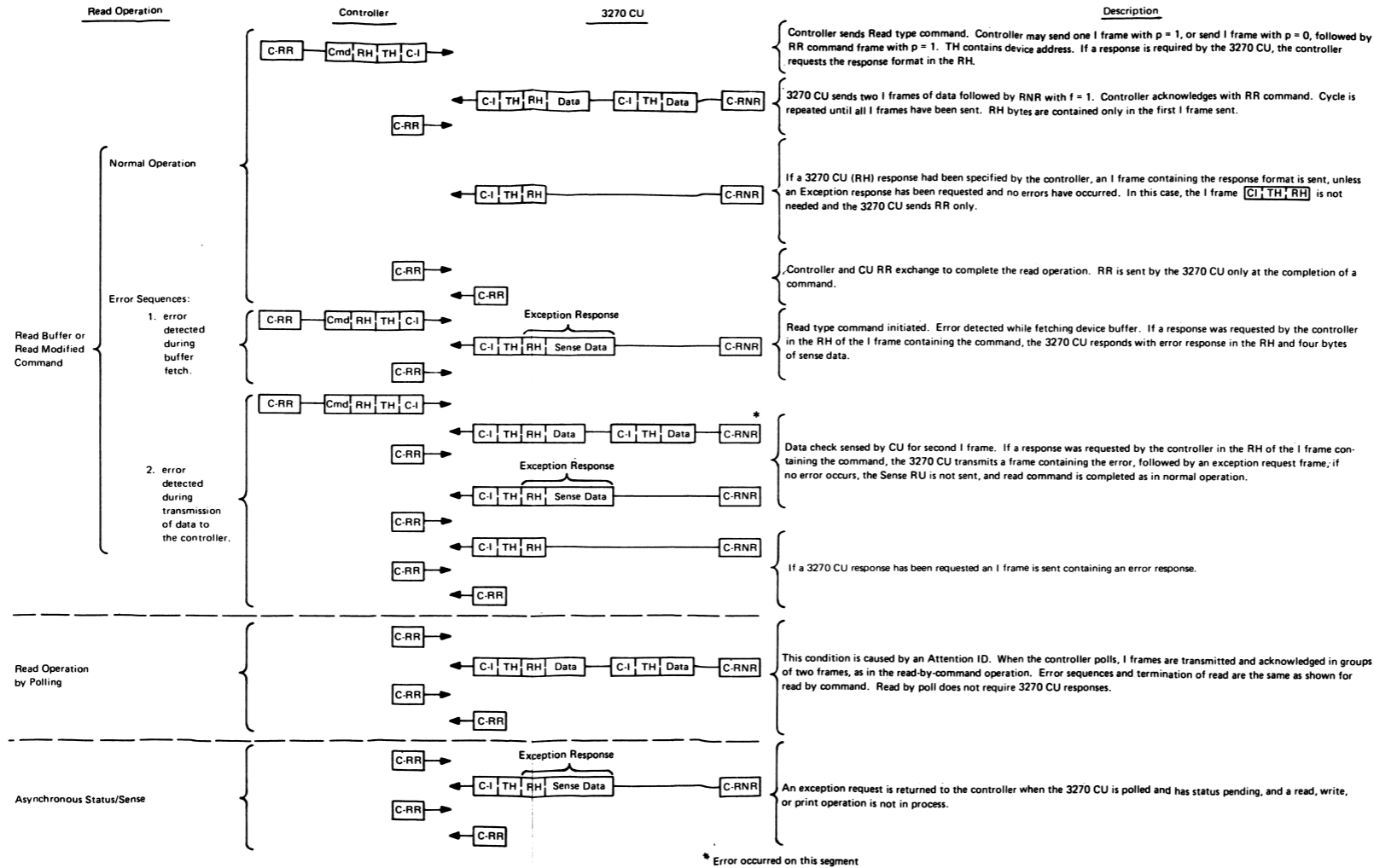
Figure 8-18. SDLC Read Type Command Sequence/Response Diagram
