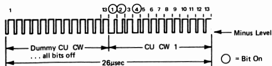
Figure 1-13. CU CW 1 Detected on 3284/3286/3288
