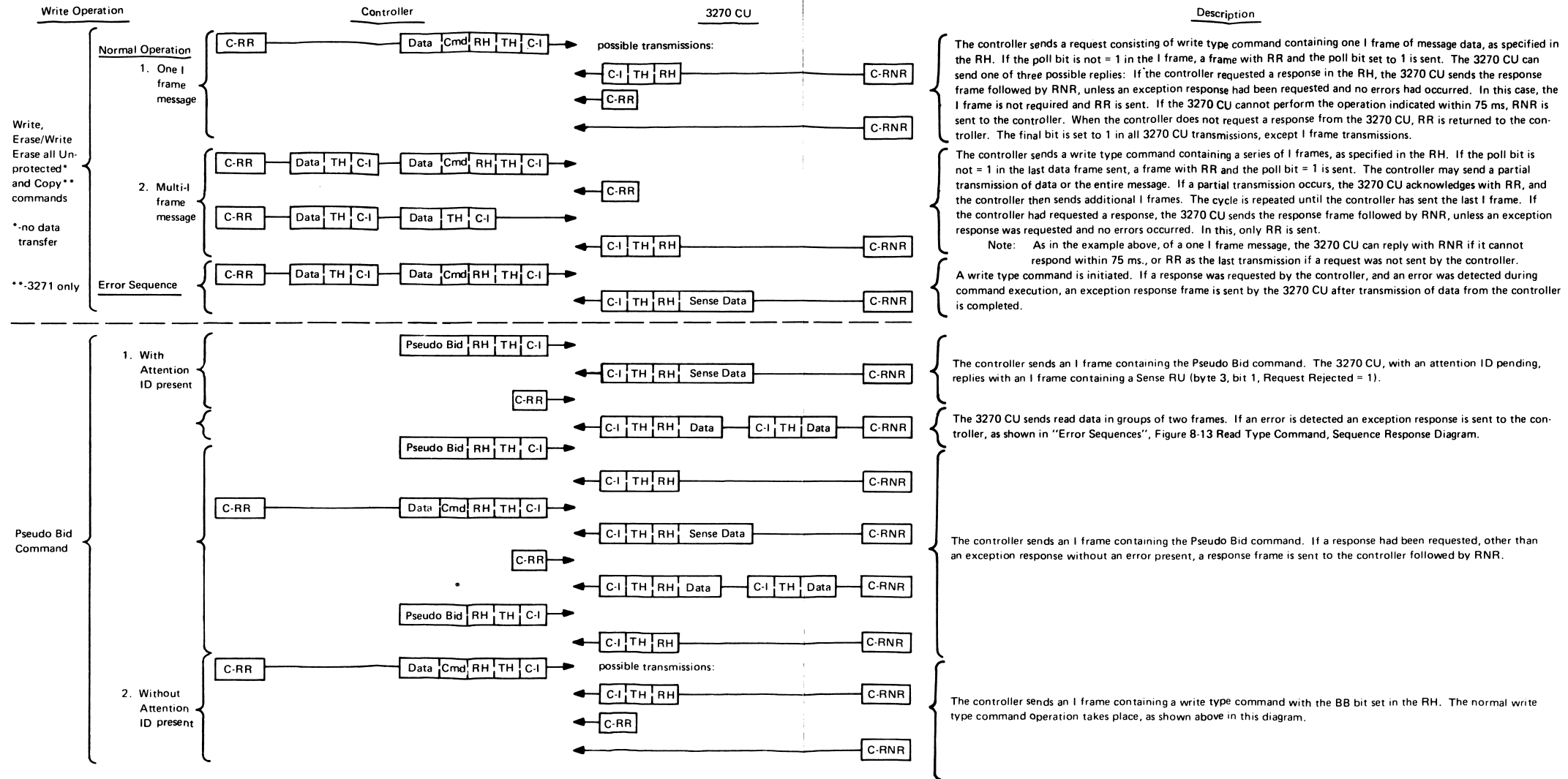
Figure 8-19. SDLC Write Type Command Sequence/Response Diagram
