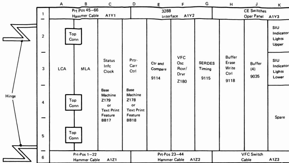
Logic Gate Front View Card Side
