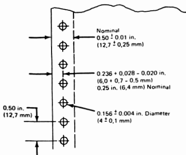
Figure 7-10. Margin Dimensions
