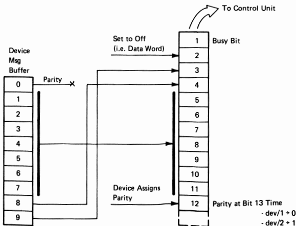
Figure 1-17. Device Buffer Transfer (Data Words) to Control Unit
