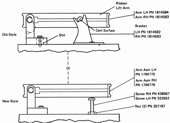
Figure 7-16. Ribbon Lift Arm Assemblies (Old and New Styles)
