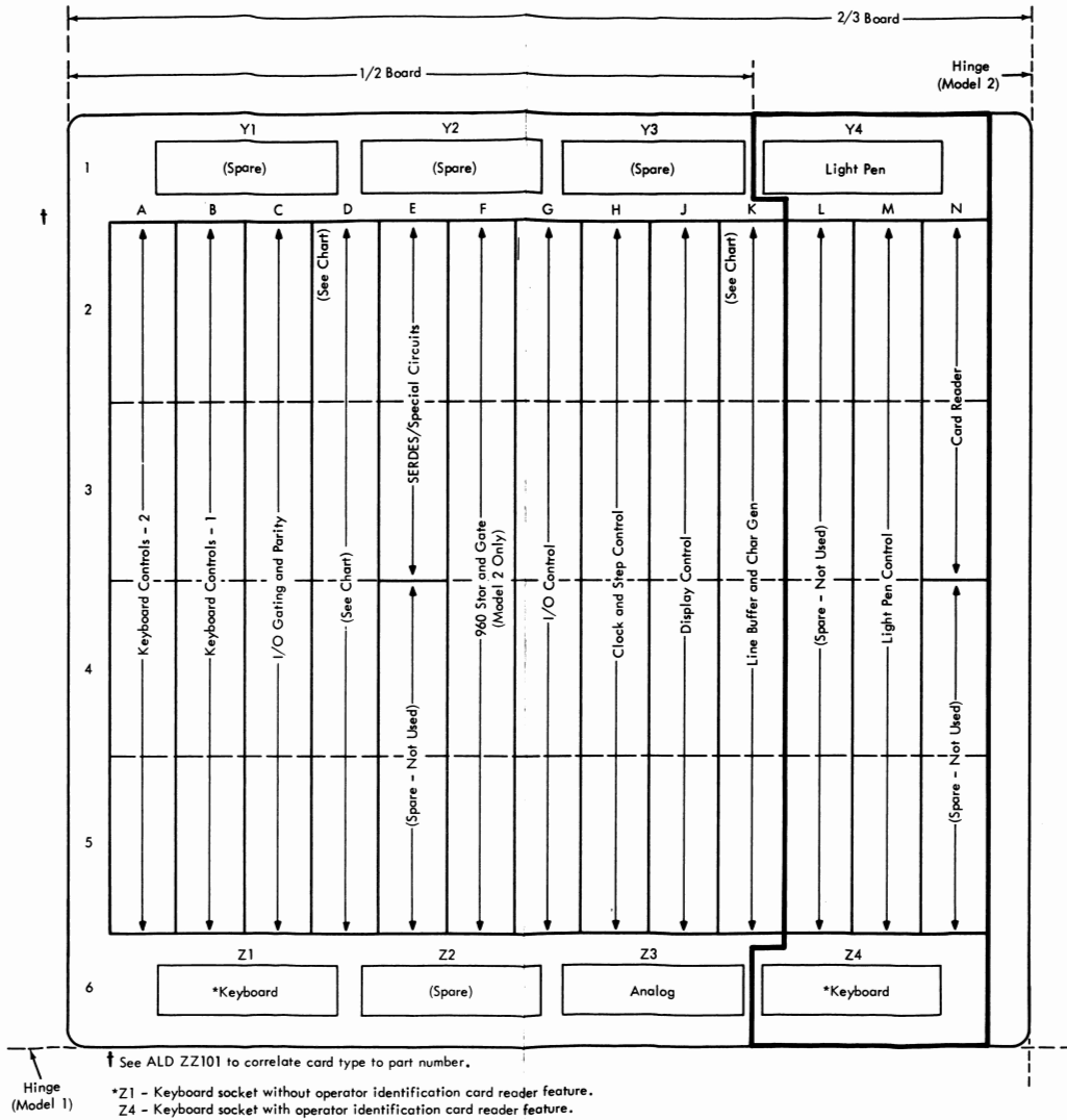
Figure 5-2. 3277 A-Gate Card Layout by Function
