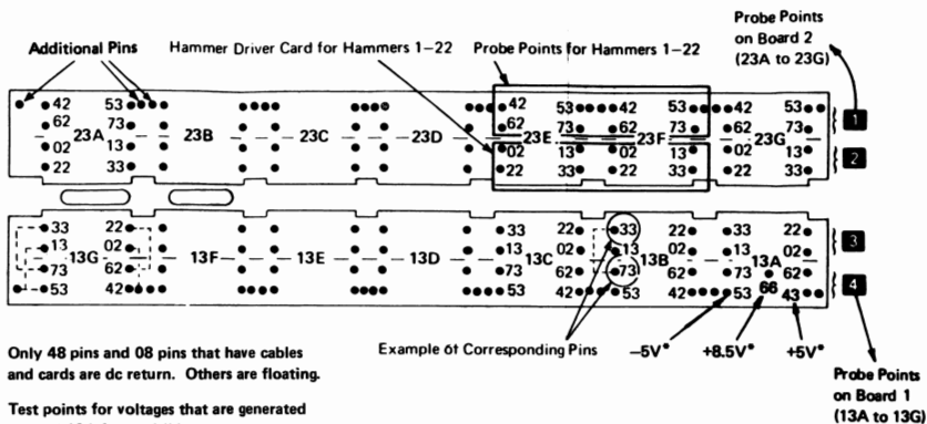
Figure 7-4. Printer Card Gate Layout
