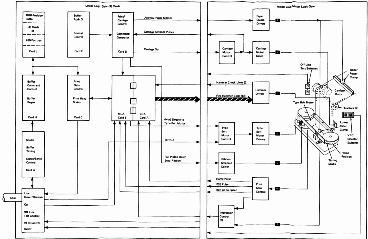
Figure 7-1. 3288 Block Diagram
