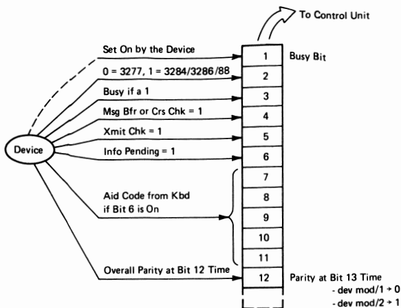
Figure 1-18. Status Word Sent by Device
