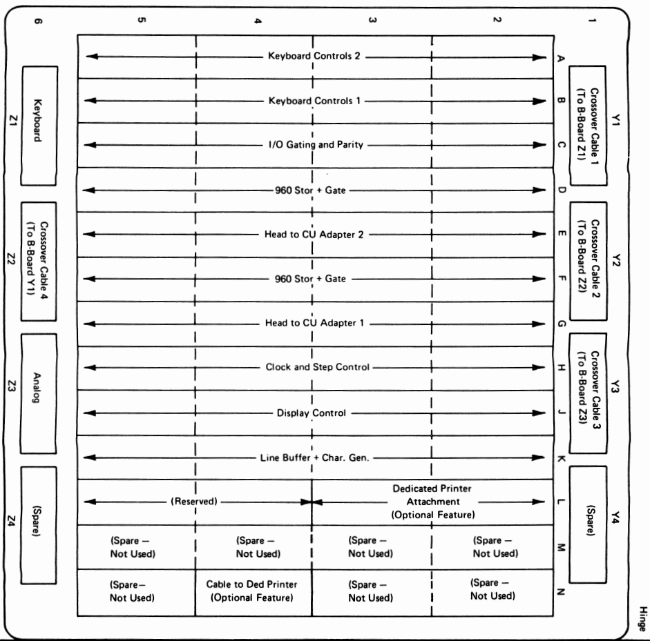
Figure 4-8. 3275 Model 3 A-Gate Card Layout by Function
