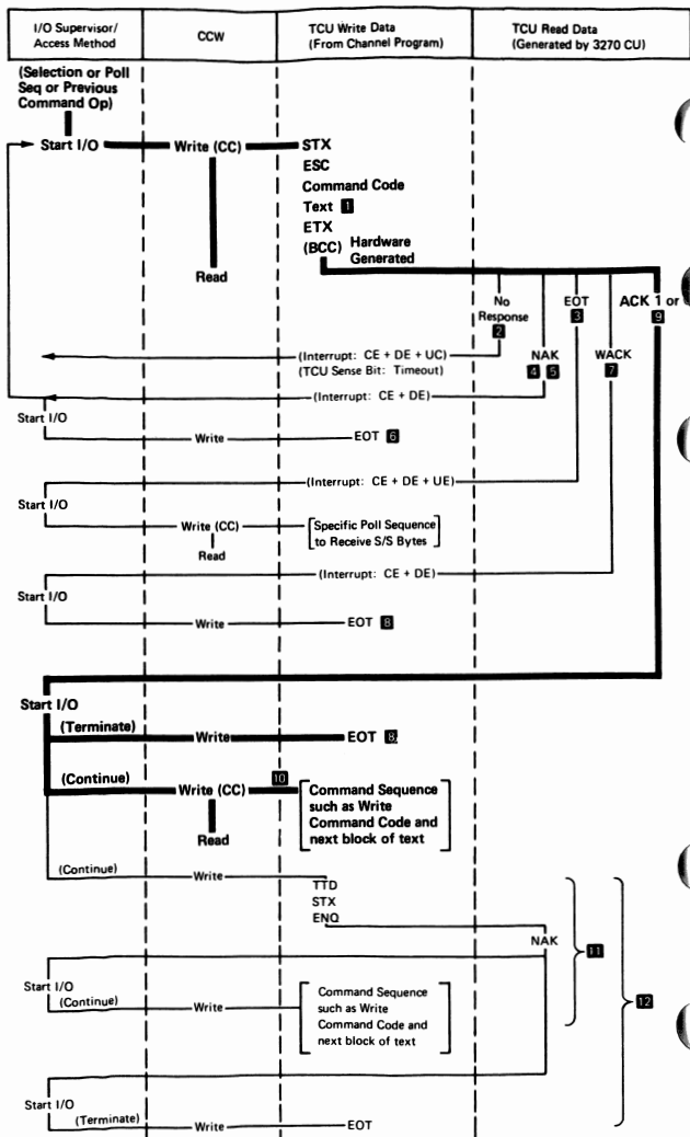
Figure 1-45 (Part 1 of 2). Write-Type and Control-Type Commands, Sequence/Response Diagram
