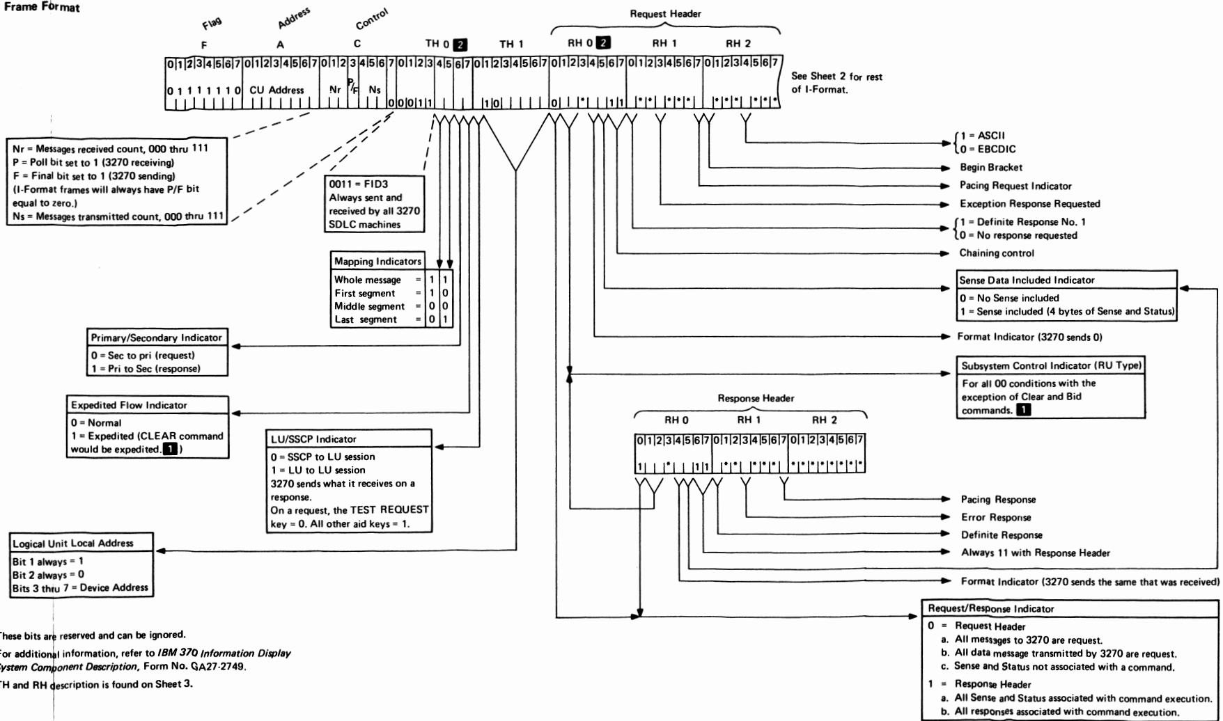
Figure 8-6 (Part 1 of 3). I-Format, Data Message
