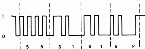
ASCII pattern every 3 sec from 3271 to TCU
