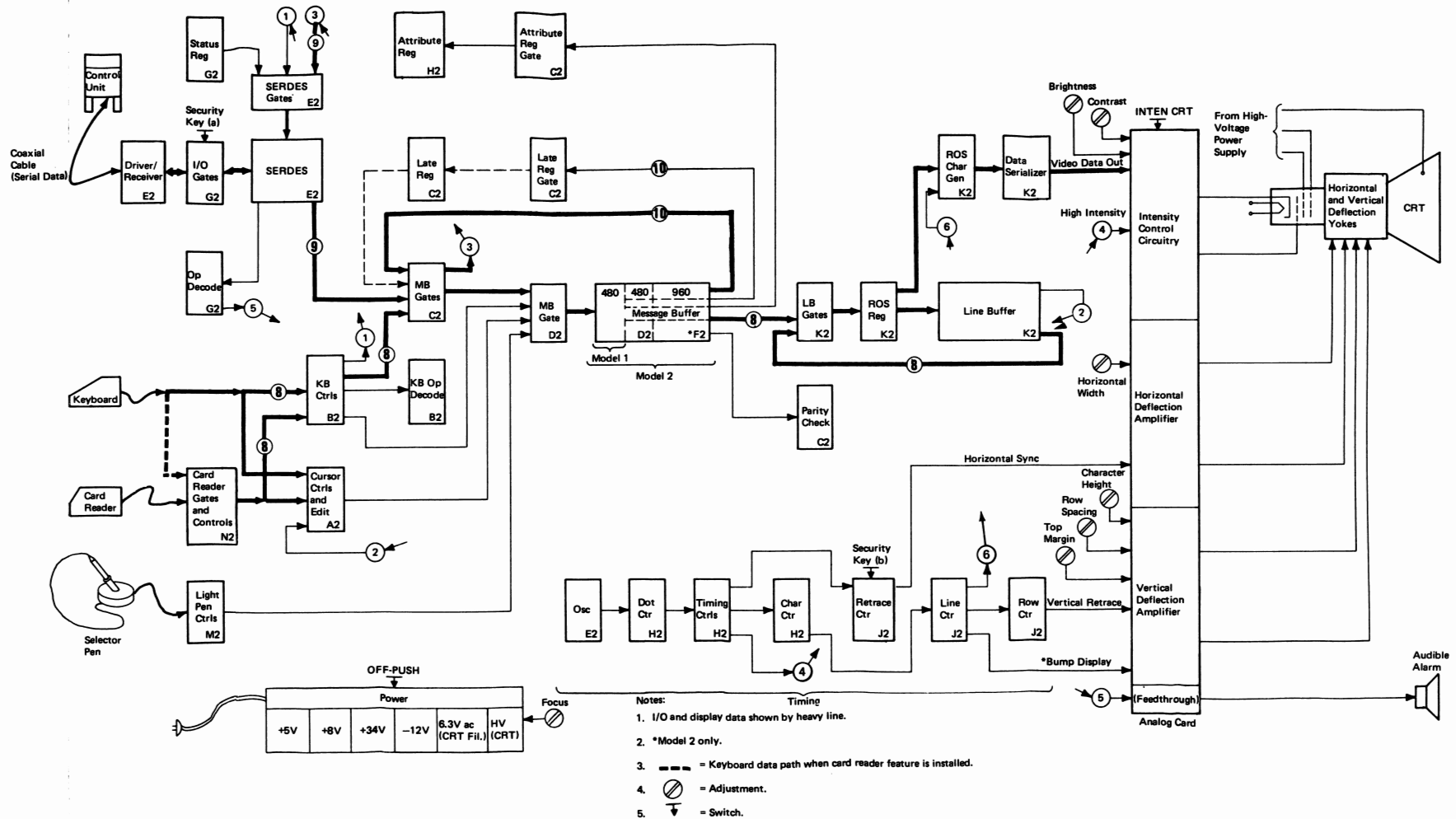
Figure 5-1. 3277 Data Flow
