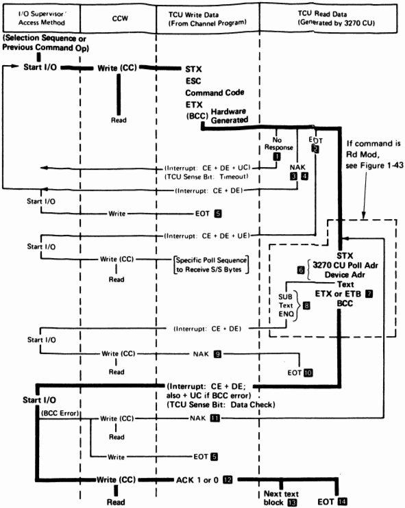
Figure 1-46 (Part 1 of 2). Read-Type Command, Sequence/Response Diagram
