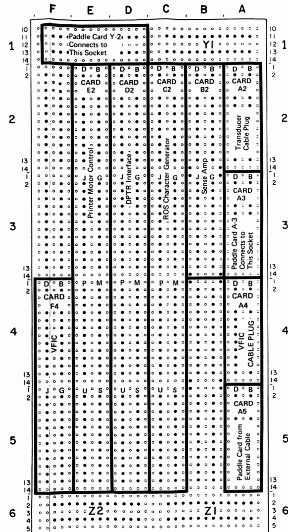
Figure 6-7. 3284/3286 Model 3 A-Gate Card Layout by Function - VFIC
