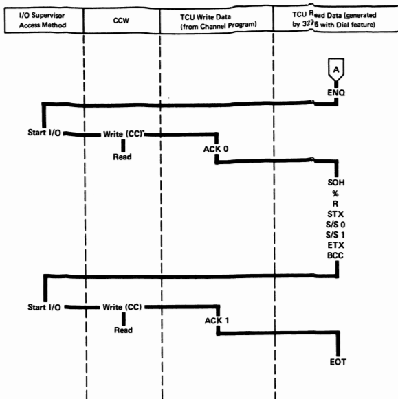
Figure 1-50. Status Message Transmission with Dial Feature, Sequence/Response Diagram
