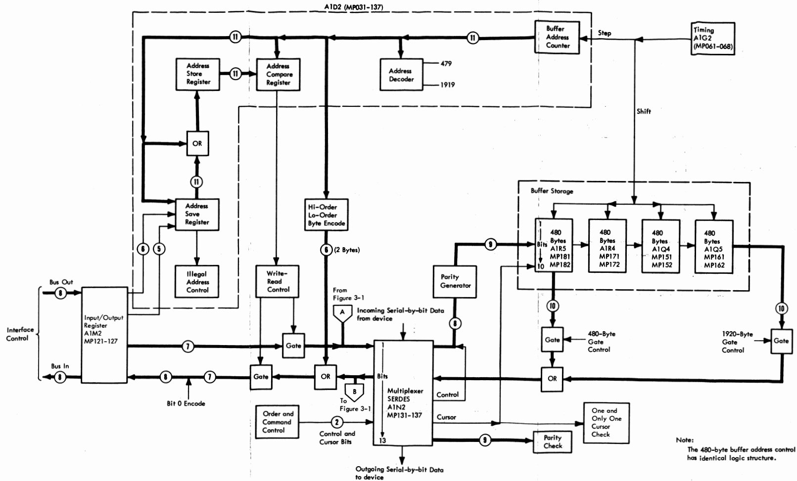
Figure 3-2. 3272 Buffer Storage Address Control
