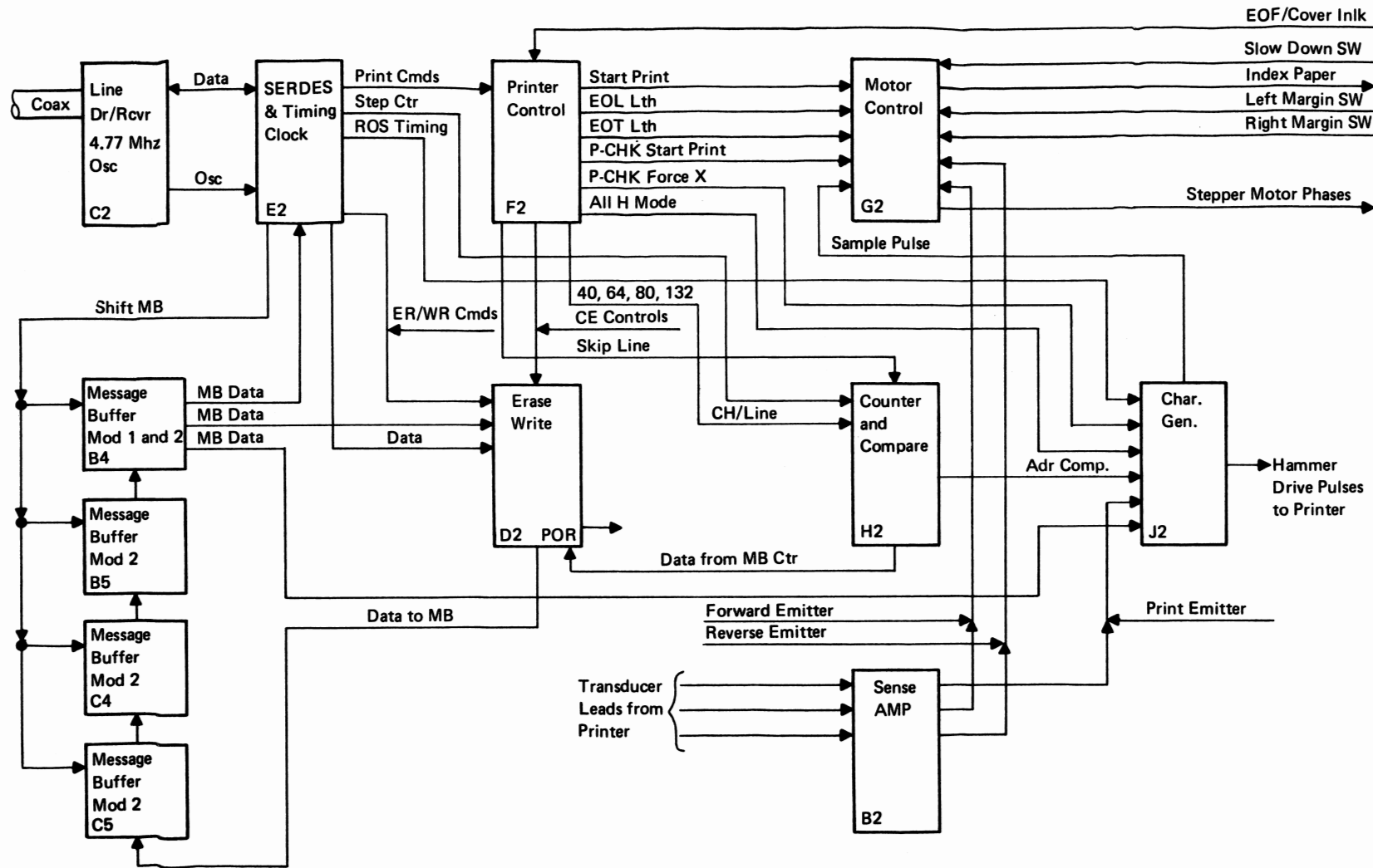
Figure 6-1. 3284/3286 Model 1 and 2 Block Diagram
