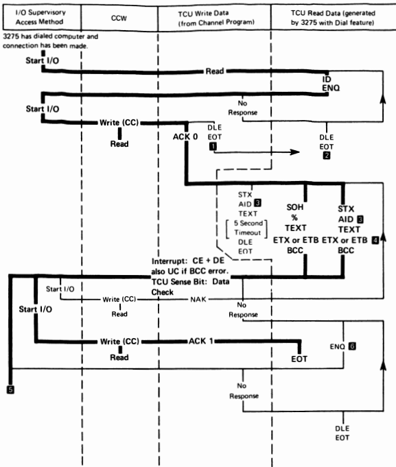
Figure 1-47 (Part 1 of 2). 3275-Initiated Transmission, Sequence/Response Diagram – Dial Feature
