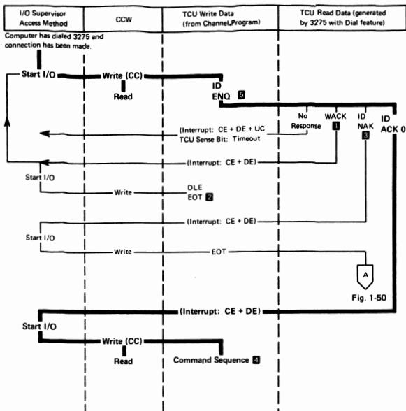
Figure 1-48 (Part 1 of 2). TCU-Initiated Transmission, Sequence/Response Diagram – Dial Feature
