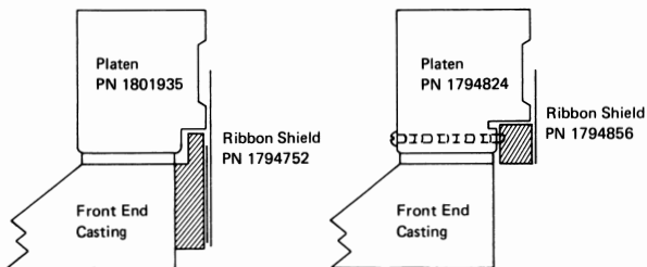
Figure 7-14. Platen/Ribbon Shield Assemblies
