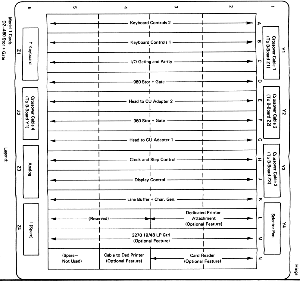
Figure 4-6. 3275 A-Gate Card Layout by Function (Display)
