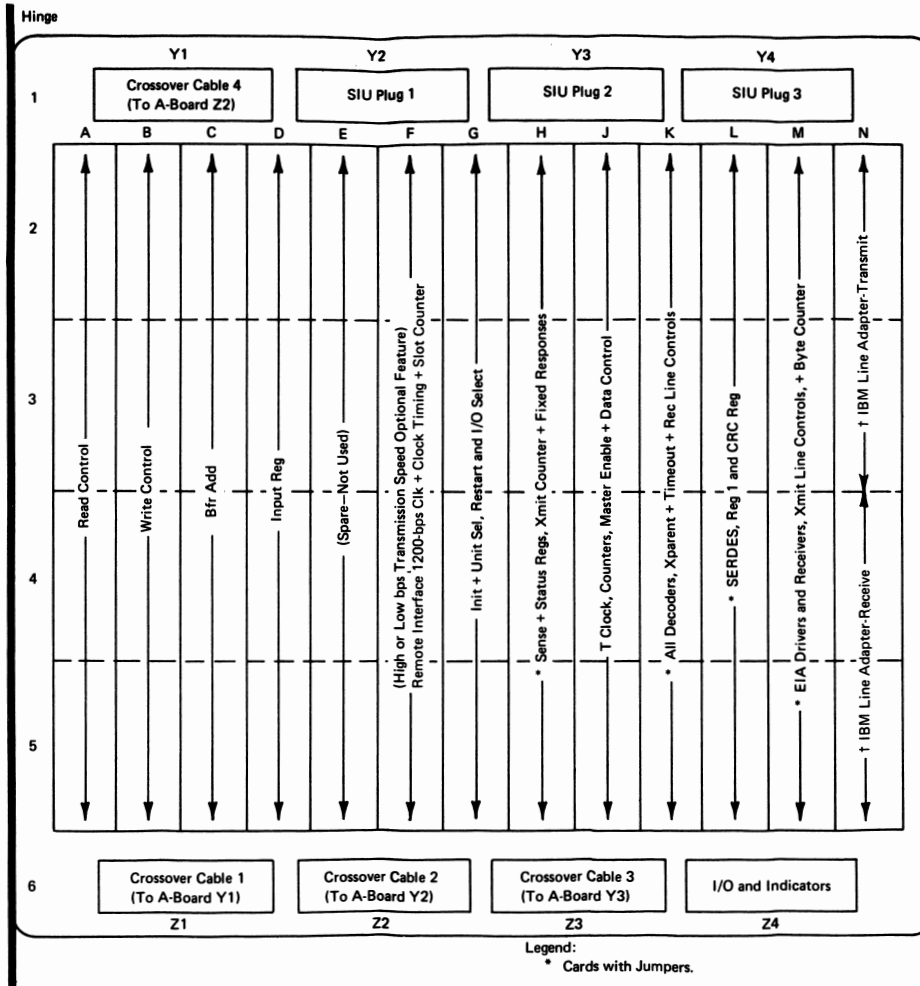
Figure 4-7. 3275 B-Gate Card Layout by Function (Leased)
