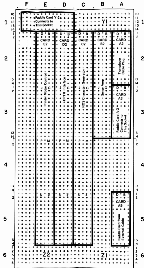
Figure 6-5. 3284/3286 Model 3 A-Gate Card Layout by Function
