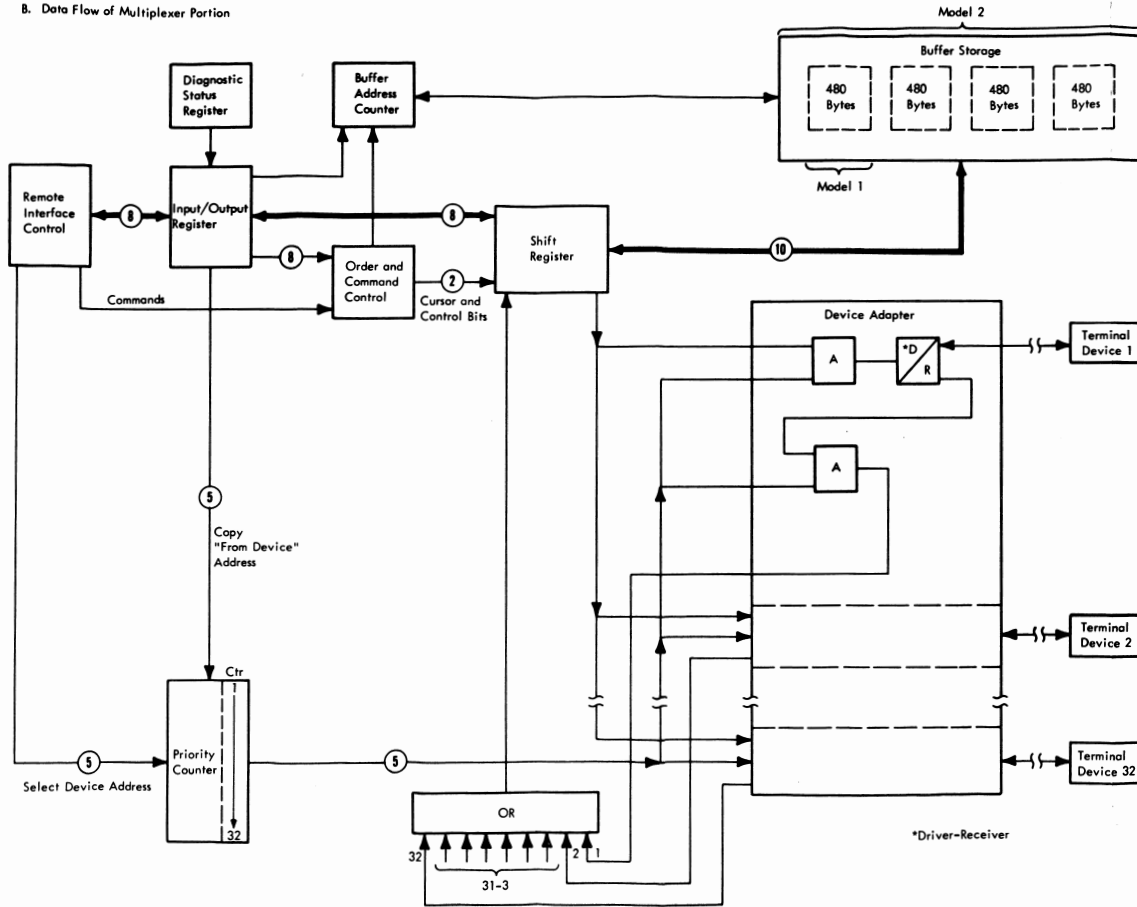
Figure 2-1 (Part 2 of 4). 3271 CU Functional Block Diagram
