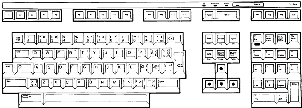
Figure B-8 Norwegian Keyboard
