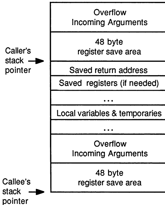
Figure 10-1. Stack Frame
